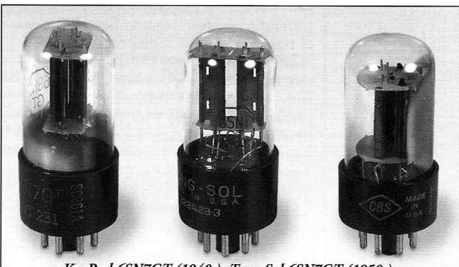
KenRad 6SN7GT (1940s), Tung-Sol 6SN7GT (1950s), CBS 6SN7GTB (1950s)
