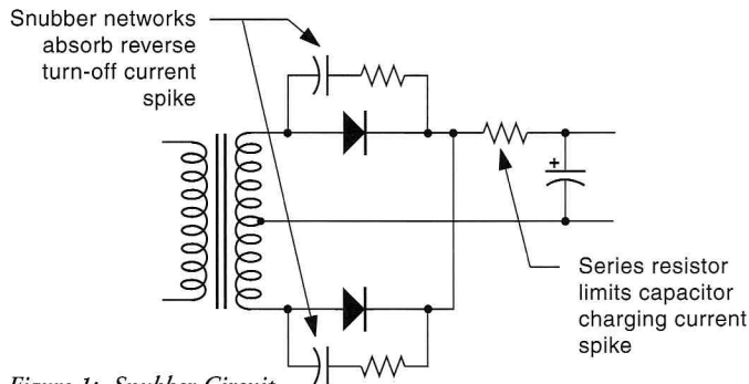
Figure 1: Snubber Circuit
