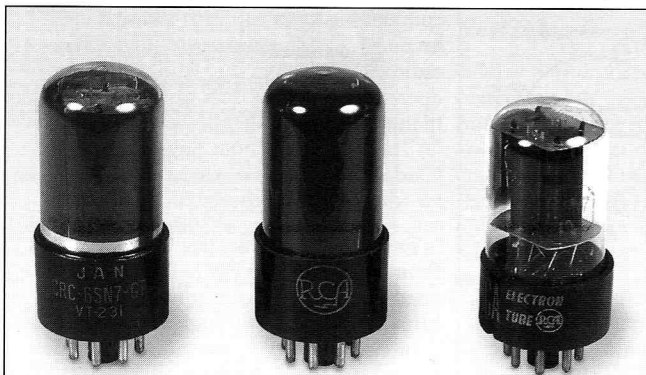
RCA 6SN7GT/VT-231 (1940s), 6SN7GT (1940s), 6SN7GTB (1960s)
