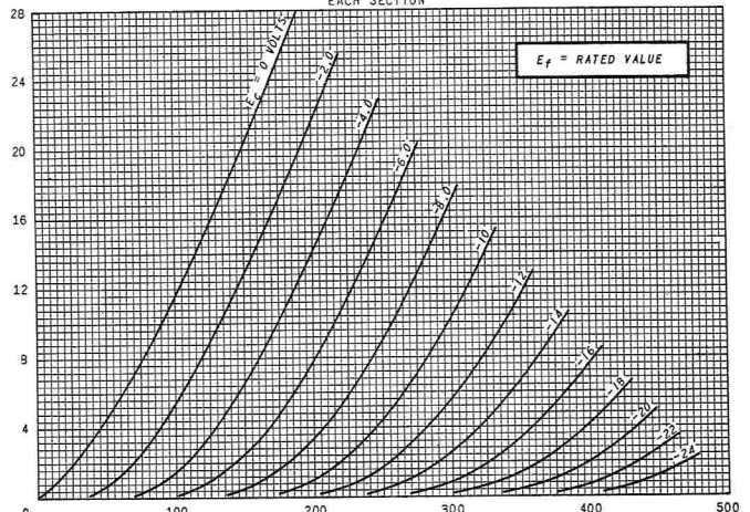
6SN7GTA AVERAGE PLATE CHARACTERISTICS EACH SECTION
