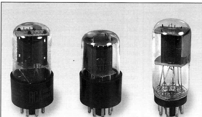
RCA 6SN7GTA (1960), GE 6SN7GTB (1960s), RCA 6SN7GTB (1975)
